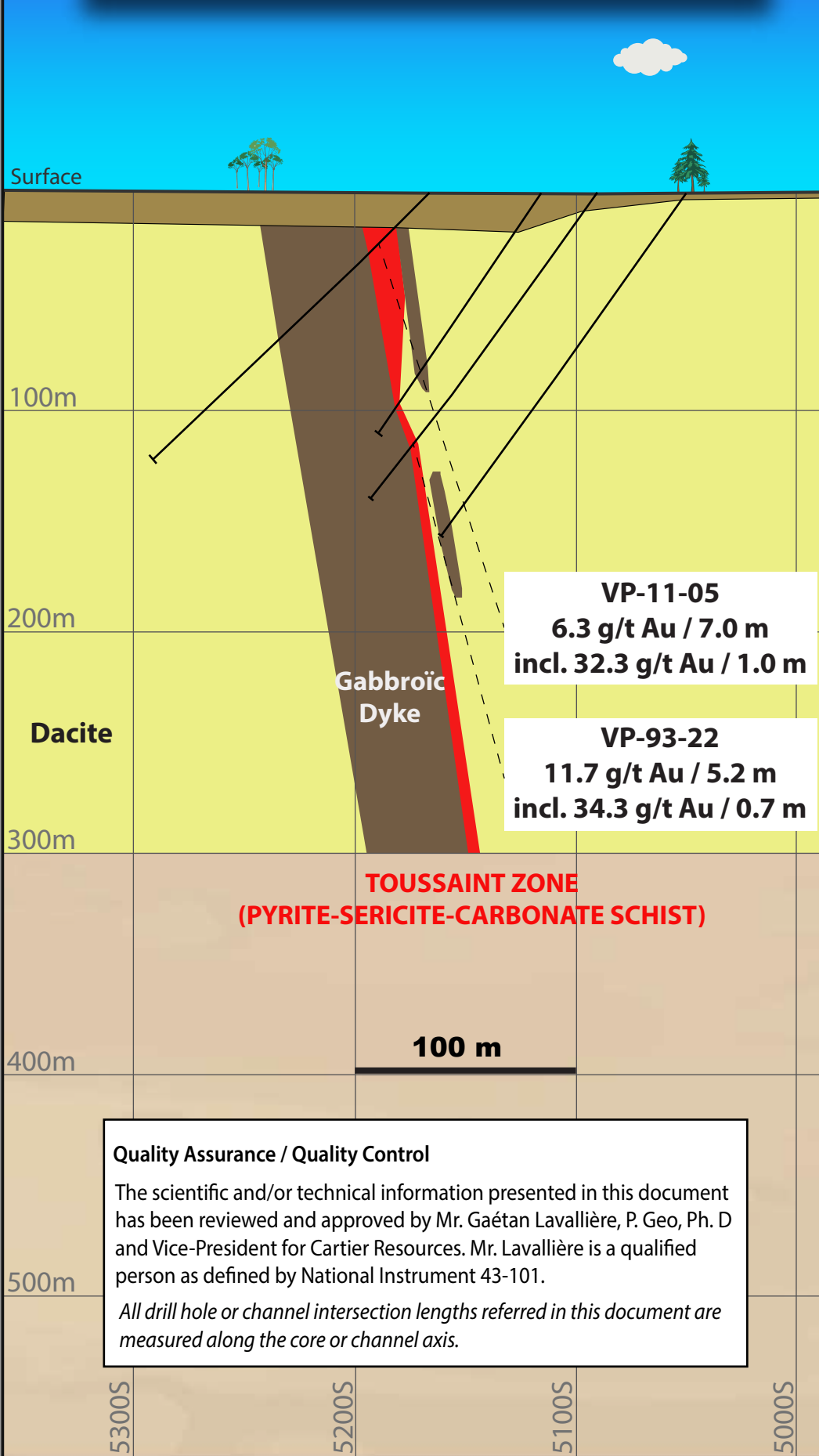
S 5440E Cross Section of Toussaint Zone (Looking West) N
